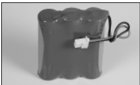
PART NO.: BATT-4165 3.6V 1500MAH NI-MH PANASONIC
