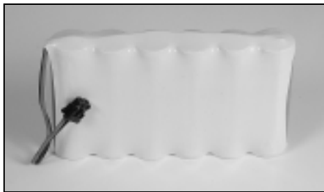
PART NO.: BATT-507 7.2V 500MAH NI-CAD PANASONIC P-P507
